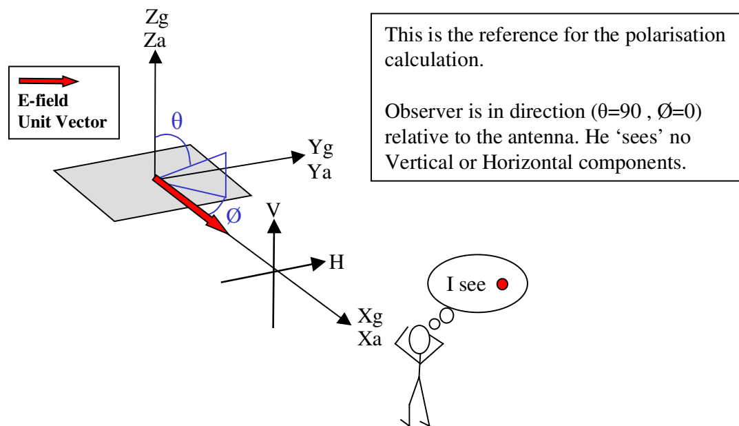
Figure 4.2-1a Polarisation Geometry 1
