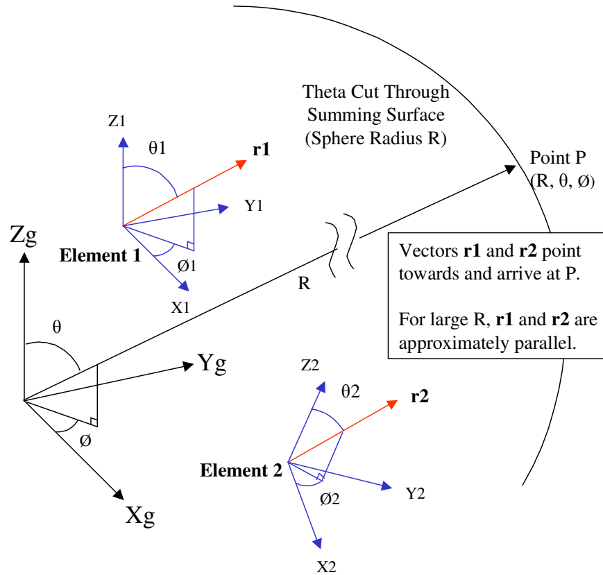
Figure 2.2-2 Array Geometry
